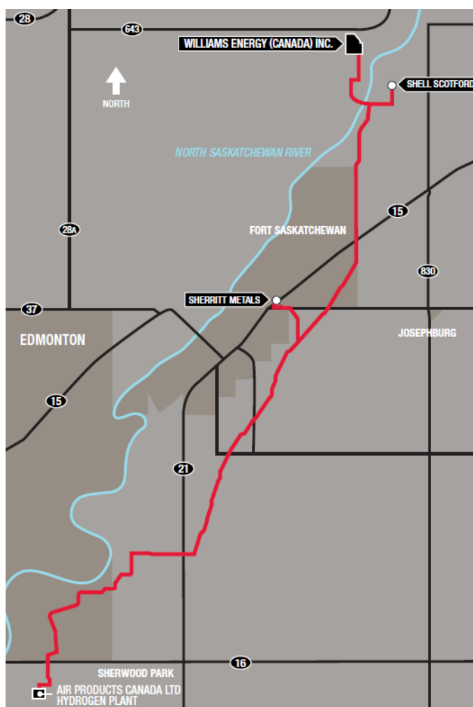
Figure 19 – Air Products Hydrogen Pipeline in Alberta
