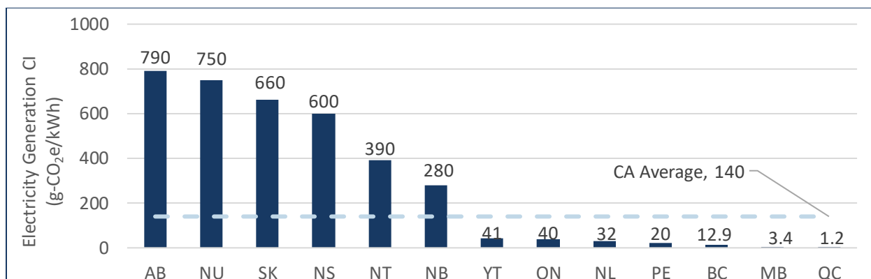
Figure 29 – Carbon Intensity of Provincial Electricity Generation Sources
