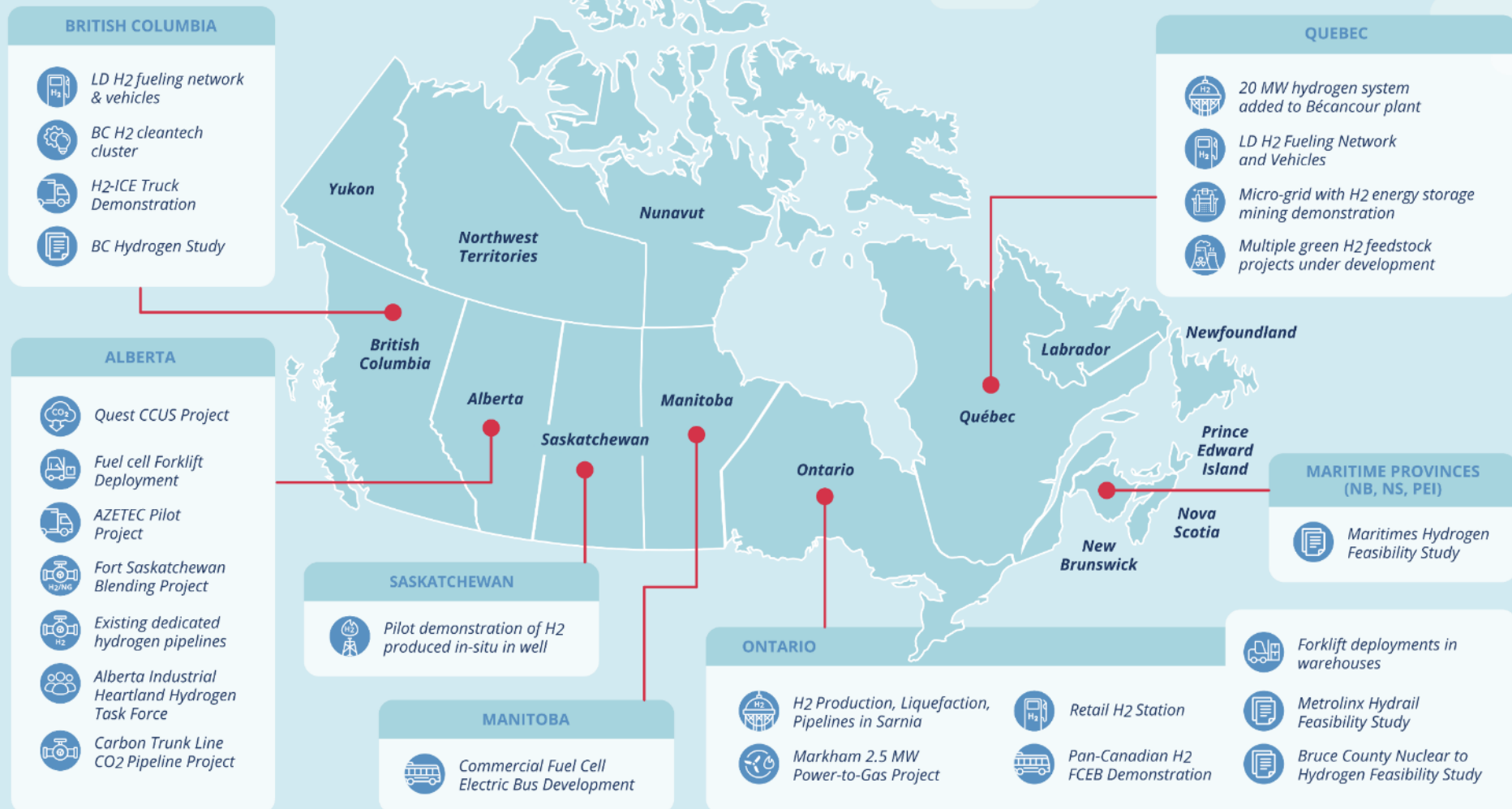
Figure 2 – Canada's Starting Point for Low-CI Hydrogen Production and Use
